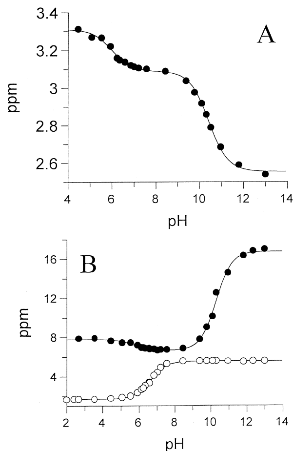
Figure 5. Titration curves for compound 4 ^1\text{H} NMR (A) and ^{31}\text{P} NMR (B) chemical shifts ( \delta , ppm) against pH are plotted. A sample of (20 mM) in \text{D}_2\text{O} was titrated between pH 2.0 and 13.0. (A), ^1\text{H} NMR chemical shifts of the methylene protons ( \text{CH}_2\text{PO}_3^{2-} ) are plotted versus pH. (B), ^{31}\text{P} NMR chemical shifts of the phosphonate ( \bullet ) and the phosphate ( \circ ) are plotted versus pH.
