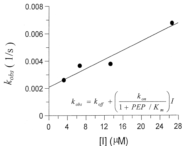
Figure 3. The plot of k_{\text{obs}} versus inhibitor ( 4 ) concentration [I] . The values of k_{\text{obs}} were obtained by fitting the progress curves of inhibition (curve B, Fig. 2) with different inhibitor concentrations (1.6–26.6 \mu\text{M} ) to the expression: A_0 - A_t = at + b e^{-kt} + c . The values of k_{\text{off}} and k_{\text{on}} were calculated from the plot and eq (2) (see insert).
