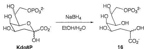
Scheme 4. Synthesis of C2-epimeric mixture of compound 16 .
