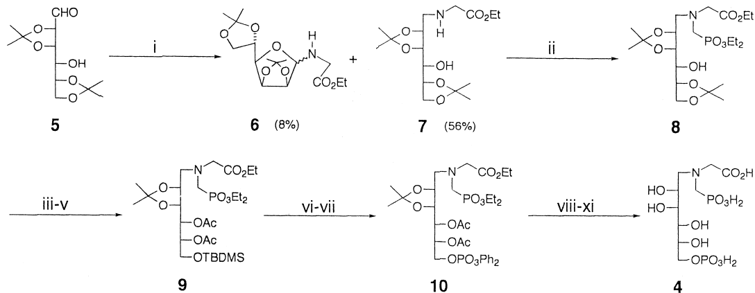
Scheme 2. Reagents and conditions: (i) H 2 NCH 2 CO 2 Et, NaBH 3 CN, MeOH; (ii) TfOCH 2 PO 3 Et 2 , sat. NaHCO 3 , CH 2 Cl 2 , 65%; (iii) TFA, MeOH/H 2 O; (iv) TBDMSCl, Py, DMAP; (v) Ac 2 O, Py, 30% over three steps; (vi) H 2 SO 4 , MeOH; (vii) (PhO) 2 P(O)Cl, Py, DMAP, 48%, two steps; (viii) TMSBr, CH 3 CN, Et 3 N; (ix) H 2 , PtO 2 , MeOH, HOAc; (x) Dowex (H + ), H 2 O; (xi) KOH, H 2 O, 35% from 10.
