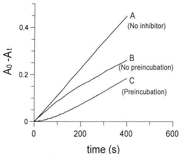
Figure 2. Progress curves for Kdo8P-synthase-catalyzed reaction in the presence of the inhibitor 4 . Curve A, the control experiment without the presence of inhibitor. Curve B, the reaction was initiated by addition of enzyme (30 nM) to the assay mixture (0.1 M Tris/HCl, pH 7.3) containing PEP (240 \mu\text{M} ), A5P (1 mM), BSA (0.1 mg/mL), and inhibitor 4 (26.6 \mu\text{M} ). Curve C, the enzyme (1.5 \mu\text{M} ) was first pre-incubated with 4 (1.33 mM) at 0^\circ\text{C} for 30 min, and then diluted 50-fold into the assay buffer pH 7.3 containing PEP (240 \mu\text{M} ), A5P (1 mM), and BSA (0.1 mg/mL). The absorbance was monitored at 232 nm.
