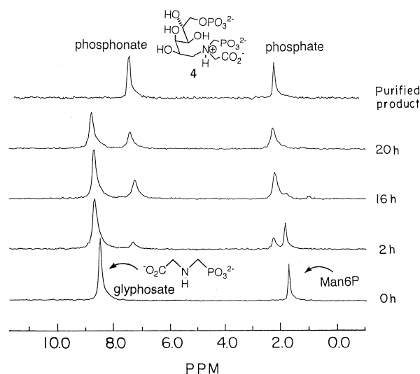
Figure 1. A timecourse of 31 P NMR spectra showing the one-step conversion of D-mannose 6-phosphate (Man6P) and glyphosate to compound 4 . The mixture of Man6P (1 equiv) and glyphosate (2 equiv) in MeOH:D 2 O (1:1) solution was treated with NaBH 3 CN (8 equiv) at pH 6.2, 80°C.
