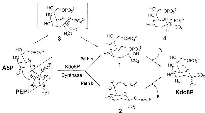
Scheme 1. Proposed mechanistic pathways for the reaction catalyzed by Kdo8P synthase.
