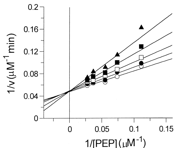
Figure 4. Inhibition of Kdo8P synthase by 4 under slow-binding conditions. Double-reciprocal plots of initial velocities are given as a function of PEP concentration when the A5P concentration was 500 \mu\text{M} , and the inhibitor concentrations were none ( \circ ), 0.0532 \mu\text{M} ( \bullet ), 0.1064 \mu\text{M} ( \square ), 0.26 \mu\text{M} ( \blacksquare ), and 0.532 \mu\text{M} ( \blacktriangle ). For the assays, the enzyme (1 \mu\text{M} ) was first preincubated with various concentrations of PEP (266–1333.3 \mu\text{M} ) and of 4 (0–17.73 \mu\text{M} ) at 0^\circ\text{C} for 30 min. The reactions were initiated by addition of aliquots (30 \mu\text{L} ) of the above preincubated enzyme mixture to the reaction buffer containing 0.1 M Tris/HCl, pH 7.3, BSA (0.1 mg/mL), and A5P (0.5 mM) at 37^\circ\text{C} .
