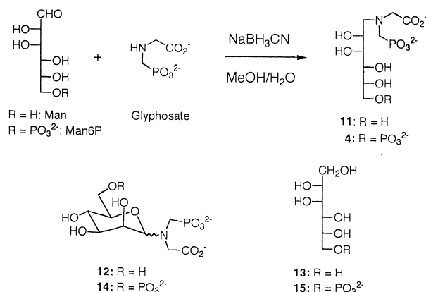
Scheme 3. One step synthesis of 4 from D-mannose 6-phosphate (Man6P) and glyphosate.
